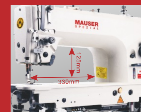
宽大的操作空间 Large operating clearance
